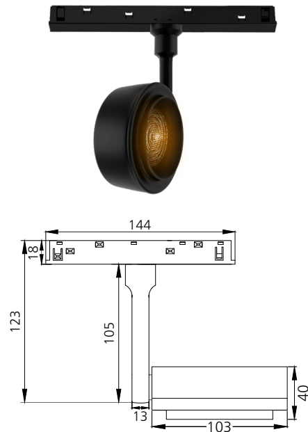
Standard - Disc M #2250
