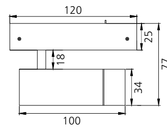
Invi M - Spot 34 #2228
