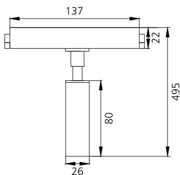
Discreet - Reading Light #2238
