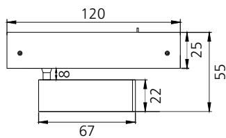
Invi S - Spot 22 #2227
