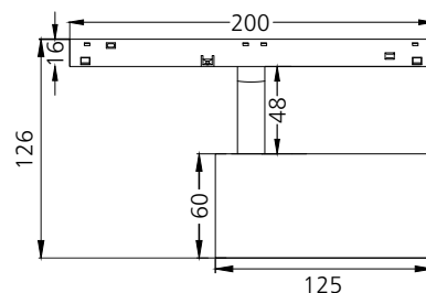
Standard L - Spot 60 #2170
