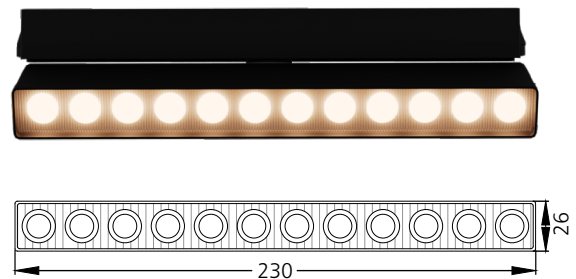
Discreet - Tilt Grid 230 #2239
