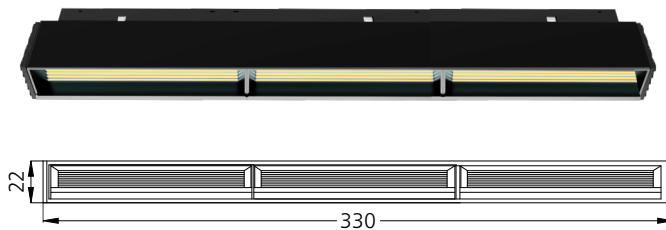
Standard L - Wash 330 #2160
