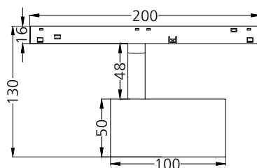
Standard M - Spot 50 #2162
