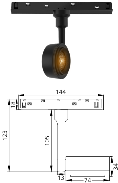
Standard - Disc S #2249
