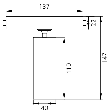
Discreet - Track Light #2237
