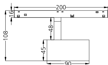
Standard S - Spot 45 #2161
